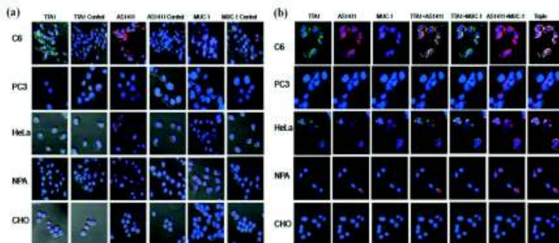
Figure 3. Confocal Microscopy Imaging of Cells Treated with QD-Aptamer Conjugates. A single incubation of QD605-TTA1, QD655-AS1411, or QD705-MUC-1 was applied to PC-3, HeLa, CHO, C6, and NPA Cells, and Confocal Images Were Obtained
