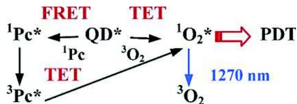
Figure 9 : Schematics of the ^1\text{O}_2 Generation in QD-based PDT Systems. Reprinted with Permission From [46].
